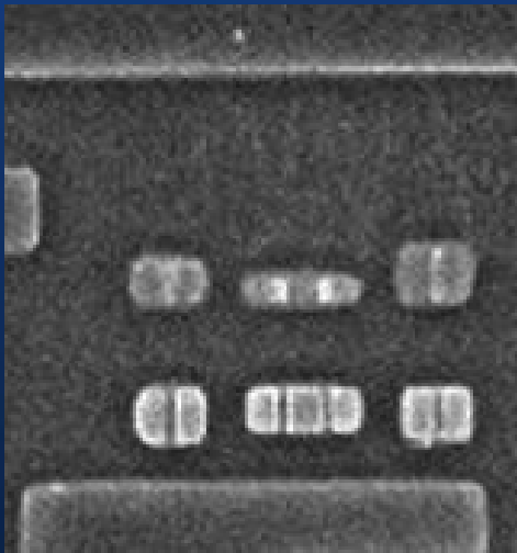
Dopant stain light = P-type dark = N-type
