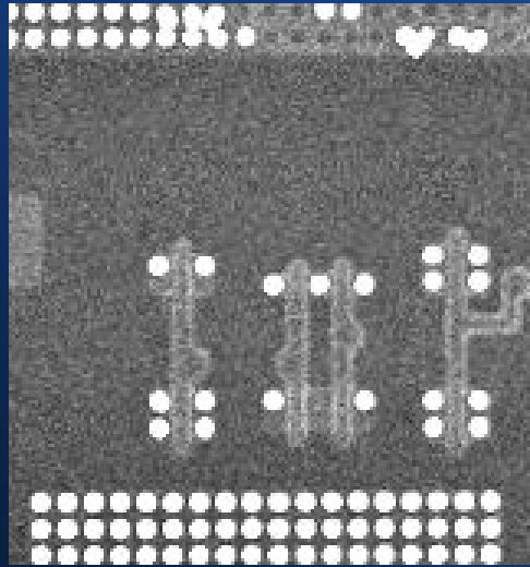
Poly + active-M1 contact Poly-M1 vias not shown
